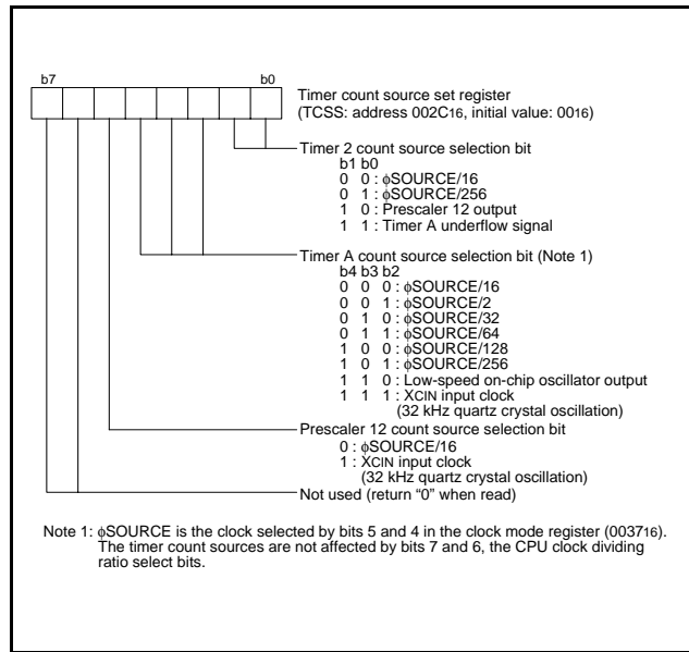
Fig 27. Structure of timer count source set register
