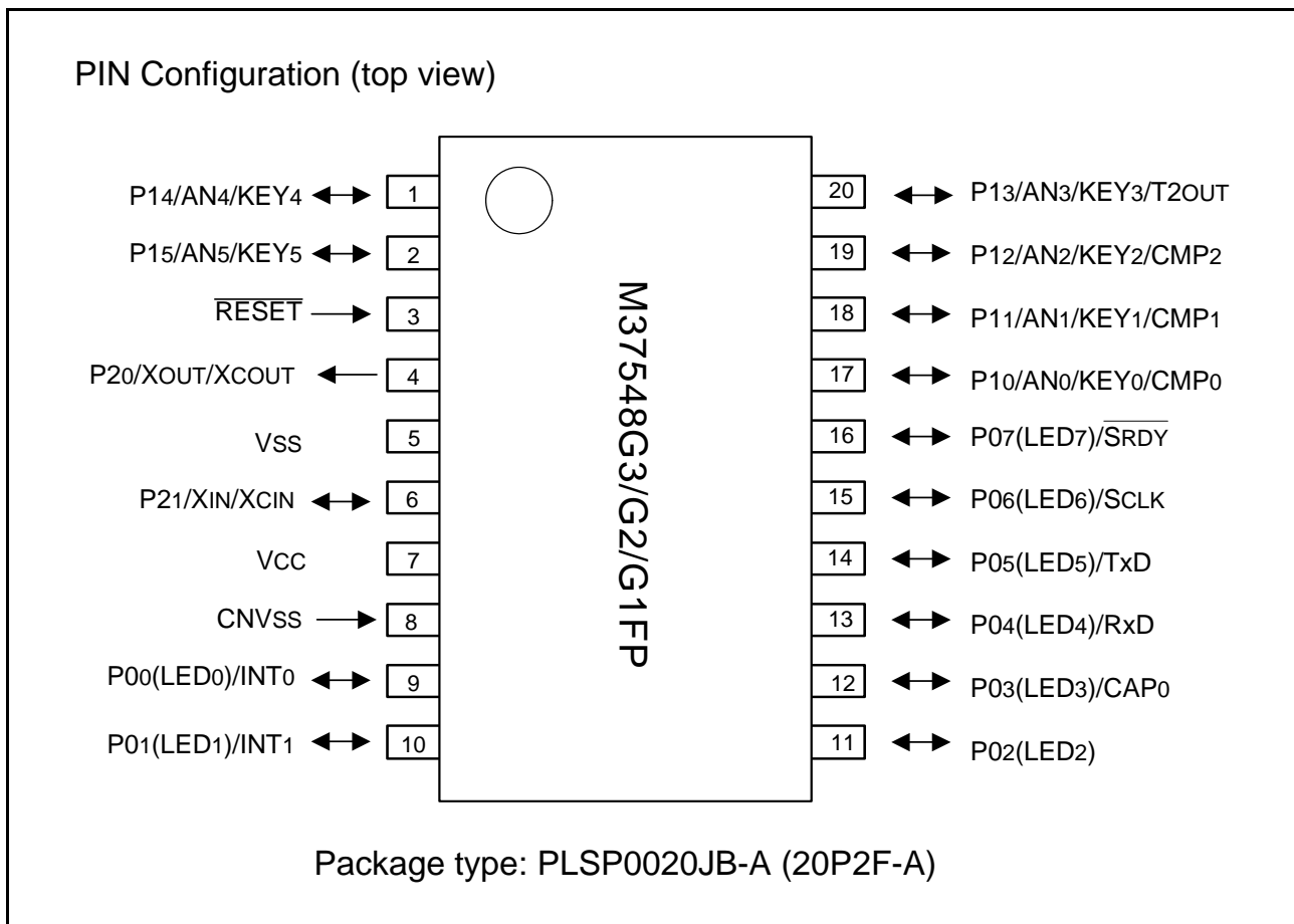
Fig 1. Pin configuration (PLSP0020JB-A type)
