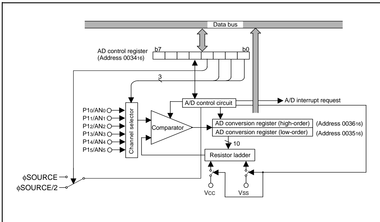
Fig 53. Block diagram of A/D converter
