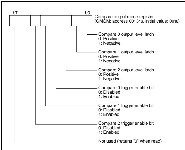
Fig 34. Structure of compare output mode register
