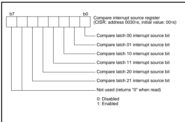
Fig 36. Structure of compare interrupt source register
