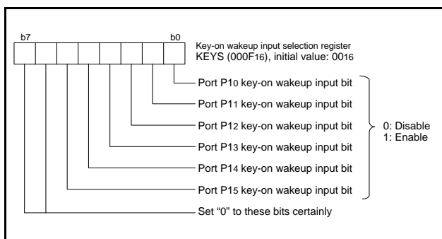
Fig 25. Structure of key input control register
