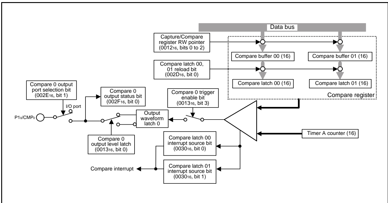
Fig 38. Block diagram of compare channel 0
