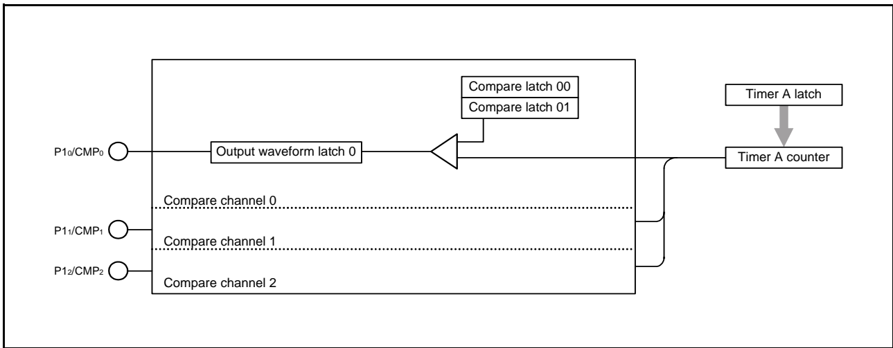
Fig 37. Block diagram of compare output circuit
