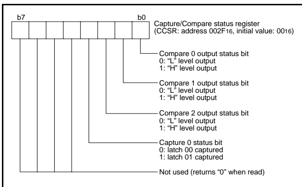
Fig 35. Structure of capture/compare status register
