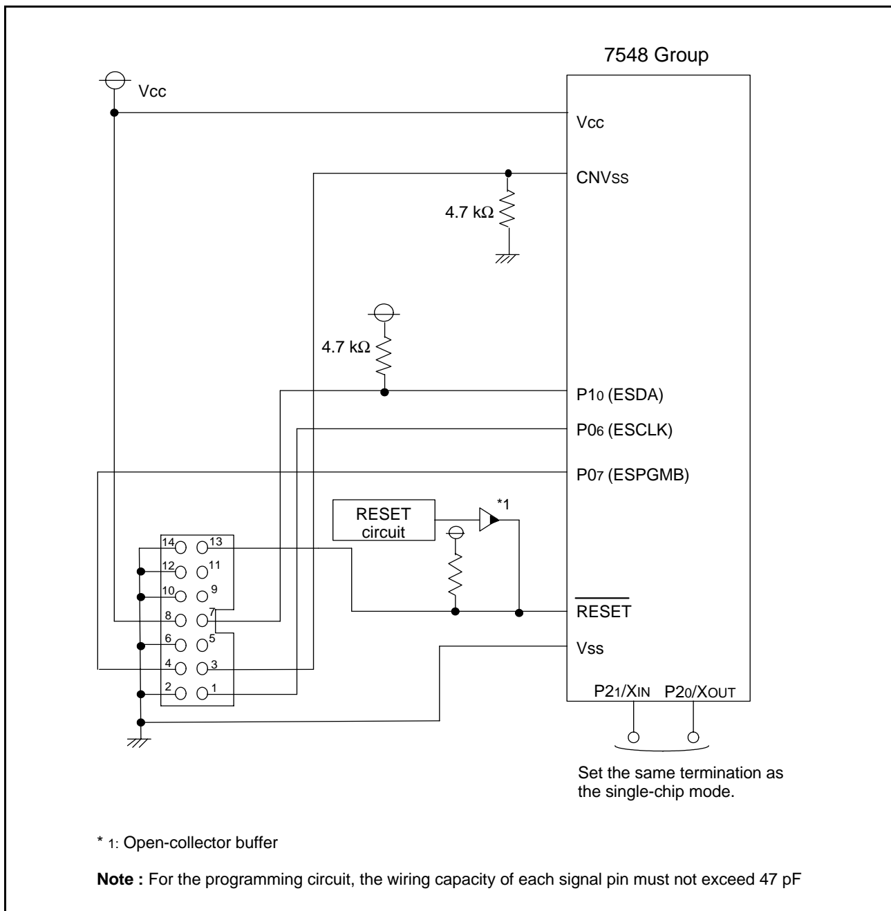
Fig 71. When using E8 programmer, connection example
