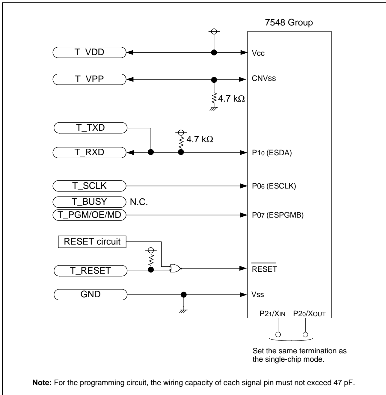
Fig 72. When using programmer of Suisai Electronics System Co., LTD, connection example
