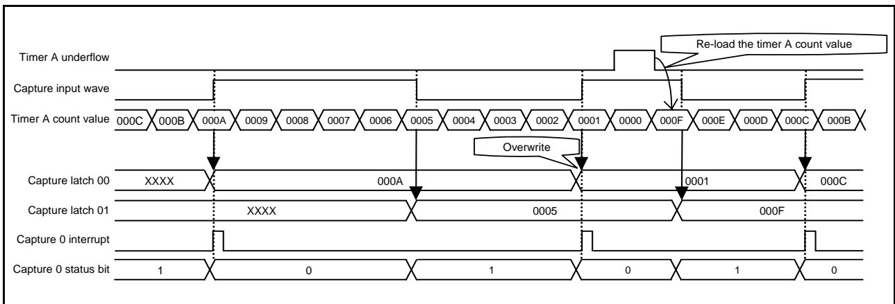
Fig 44. Capture input waveform (capture interrupt edge selection bit = "rising edge")
