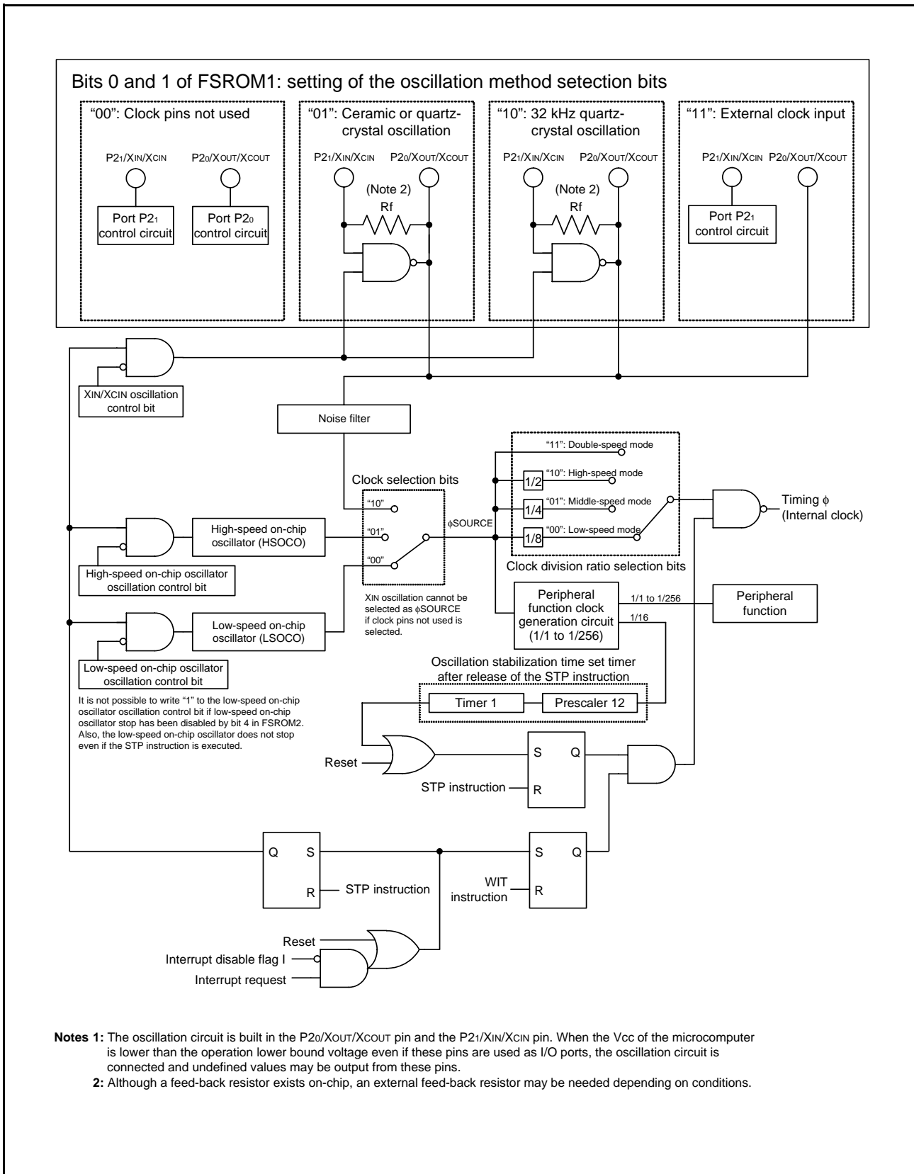
Fig 66. Block diagram of internal clock generating circuit
