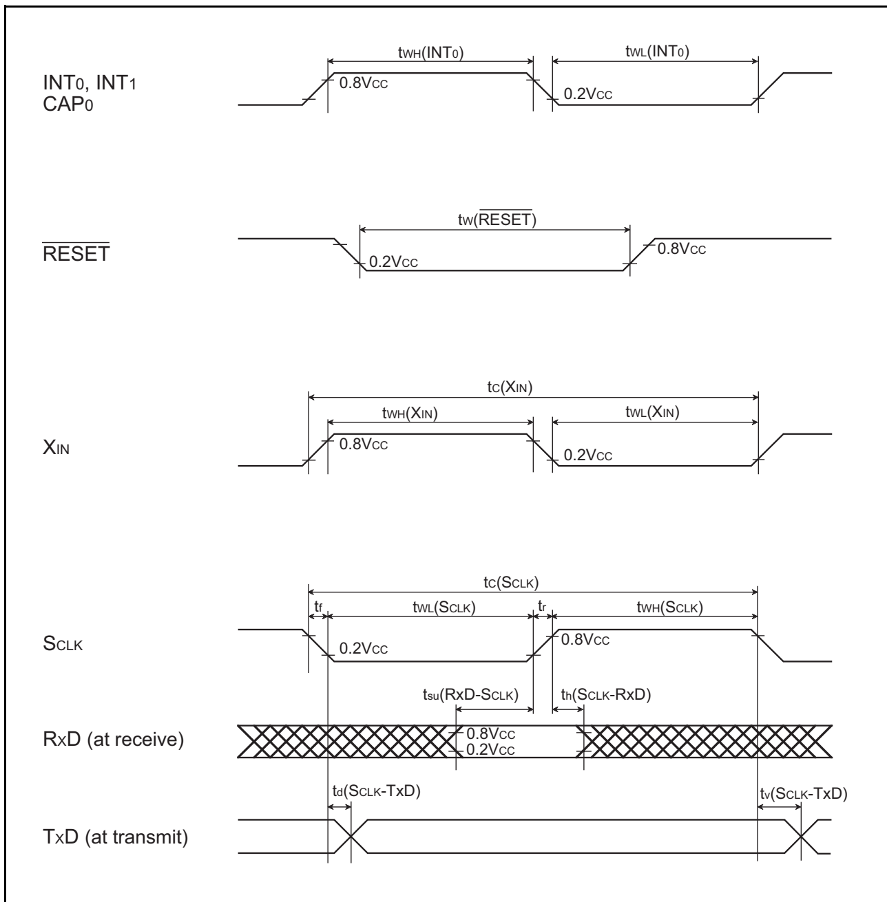
Fig 86. Timing chart
