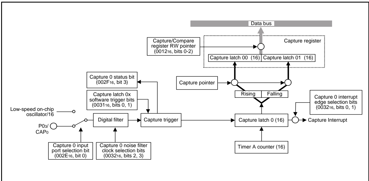
Fig 43. Block diagram of capture channel 0
