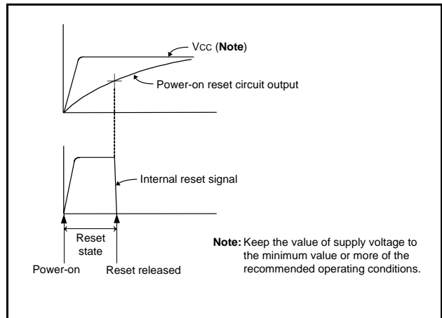
Fig 57. Operation waveform diagram of power-on reset circuit
