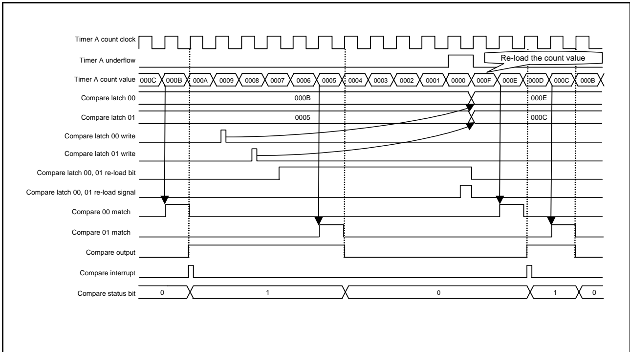
Fig 40. Output compare mode (compare register write timing)
