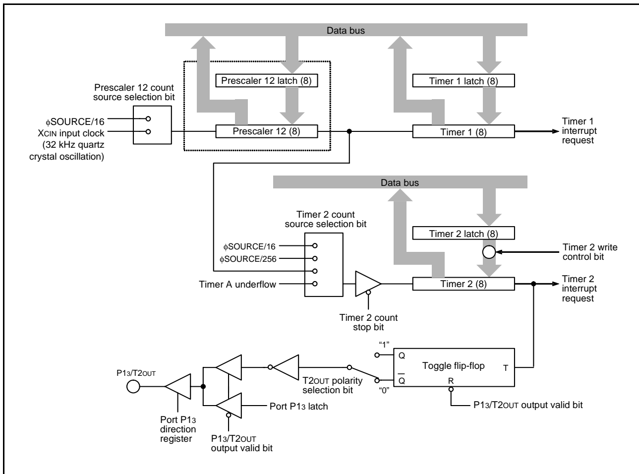
Fig 28. Block diagram of timer 1 and timer 2
