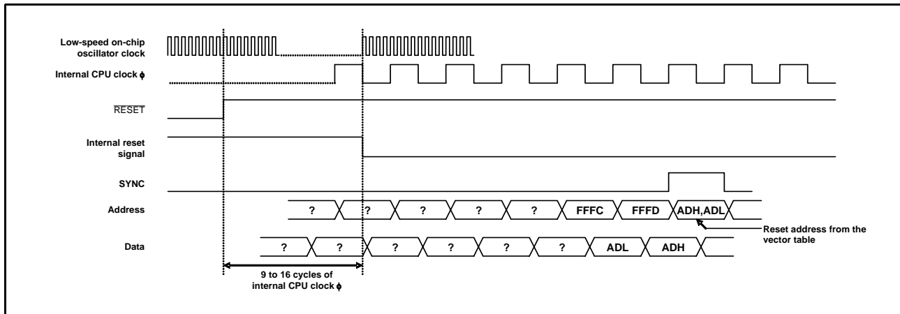
Fig 59. Timing diagram at reset
